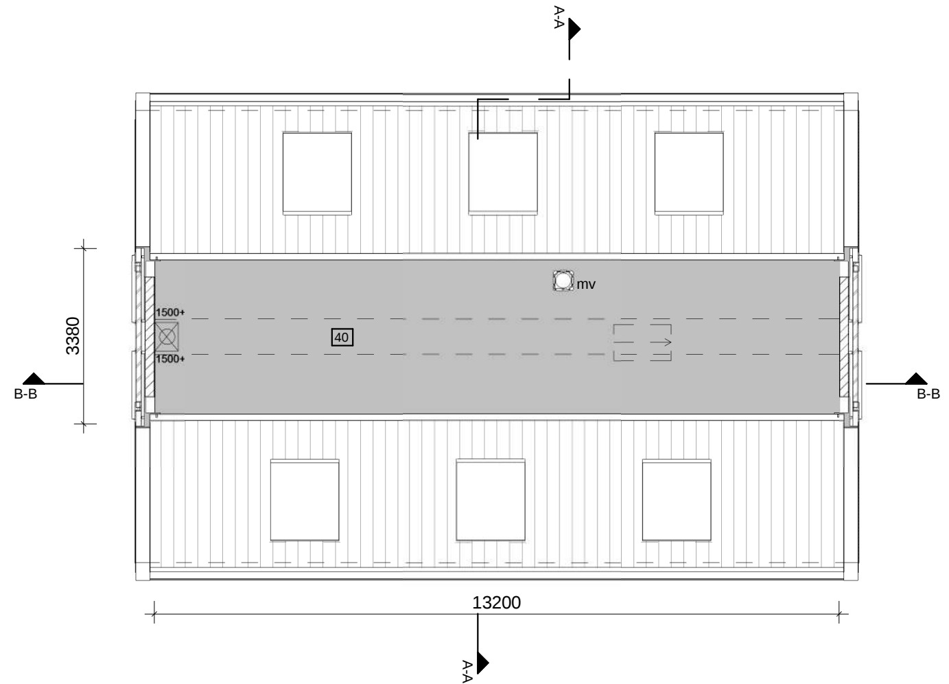
zolder
